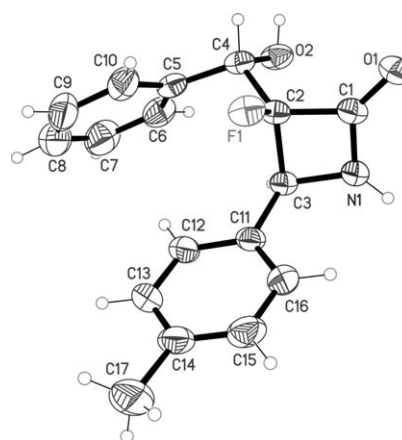
Figure 2. ORTEP structure of lactam 8 .
