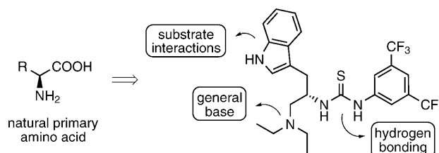
Scheme 1. Thiourea catalyst based on a primary amino acid (tryptophan).
