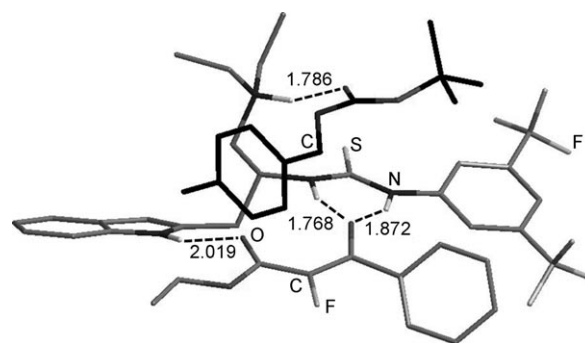
Figure 1. Intermediate IMA formed from 1a , 2a , and Trp-1 . Hydrogen-bond distances are given in Å (non-hydrogen-bonded hydrogen atoms were omitted for clarity).
