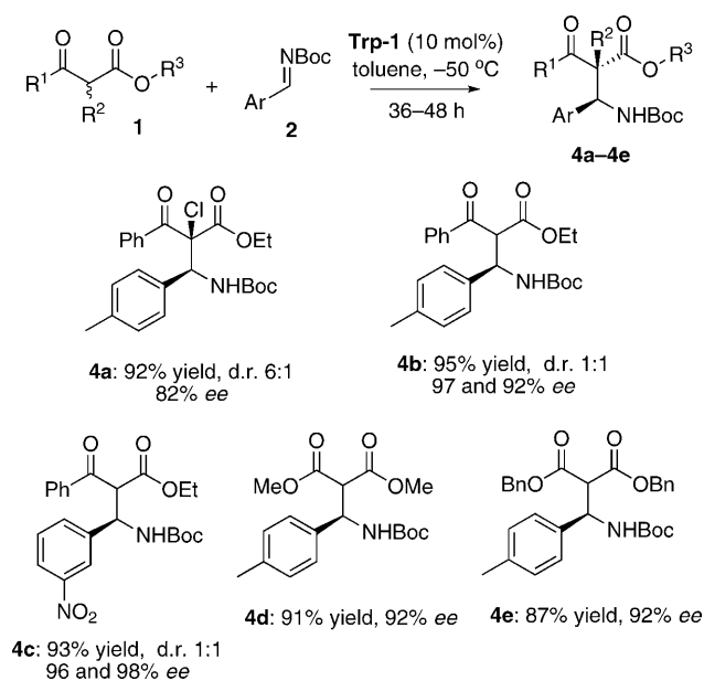
Scheme 2. Mannich reaction of other ketoesters and malonates. Bn = benzyl.
