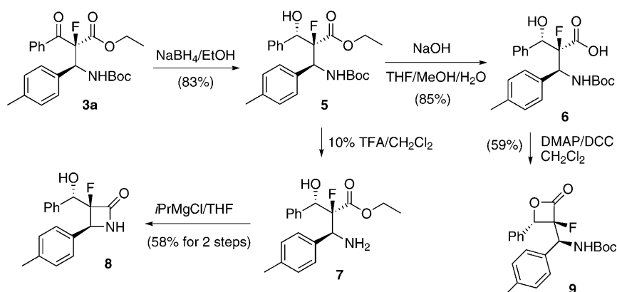
Scheme 3. Preparation of the \alpha -fluorinated \beta -amino acid 6 and \beta -lactam 8 . DCC = N,N' -dicyclohexylcarbodiimide, DMAP = 4-dimethylaminopyridine, TFA = trifluoroacetic acid.
